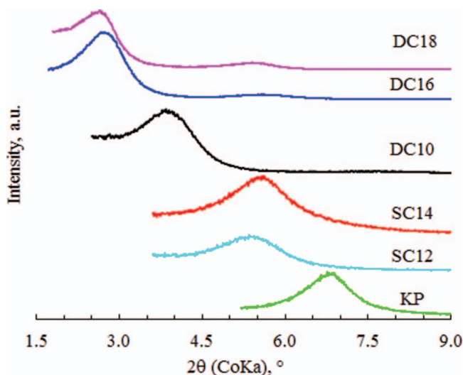
Figure 1. XRD diffractograms of crude Koppies clay and organic derivatives.
