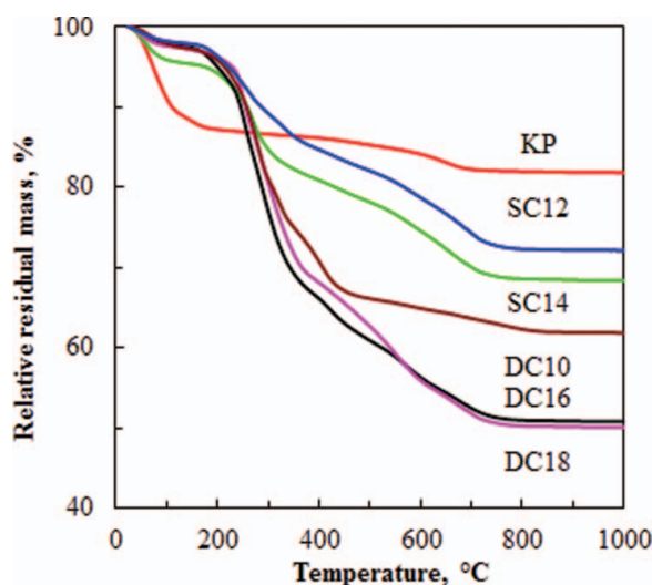
Figure 2. TG curves of crude Koppies clay and organic derivatives.
