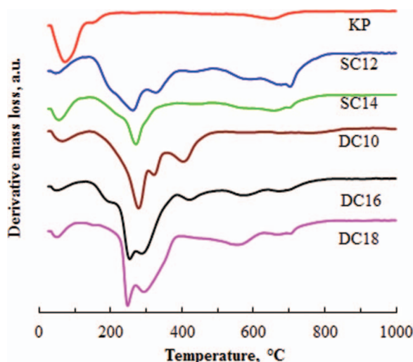
Figure 3. DTG curves of crude Koppies clay and organic derivatives.
